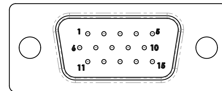
15 WAY HIGH DENSITY SUB-D CONNECTOR (PLUG) FITTED TO REAR OF LENS.
